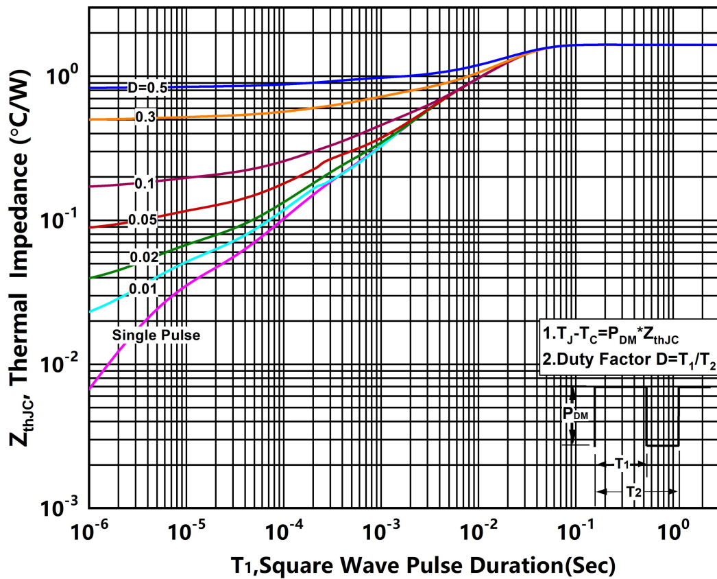
Figure.12 Transient Thermal Impedance (Junction - Case)
