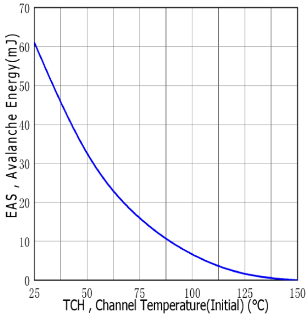
Figure.9 Maximum EAS vs Channel Temperature
