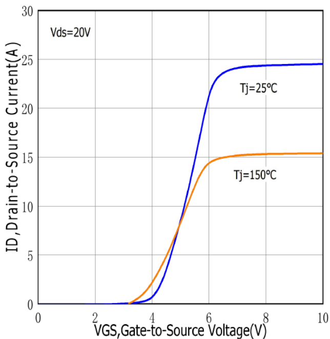
Figure.11 Typical Transfer Characteristics
