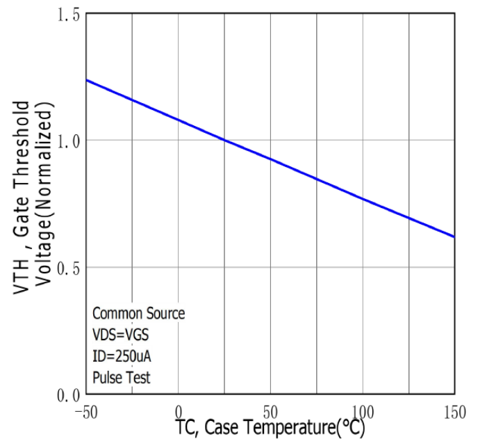
Figure.10 Typical Threshold Voltage vs Case Temperature
