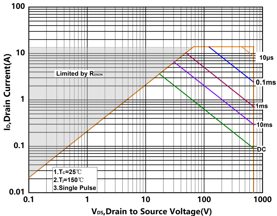
Figure.12 Safe Operating Area
