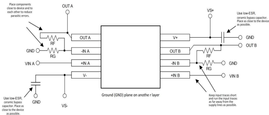
Figure 8. Layout Example
