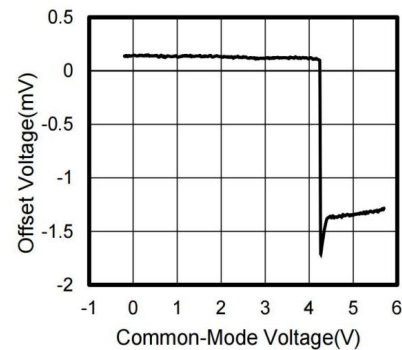
Figure 5. Offset Voltage vs Common-Mode Voltage
