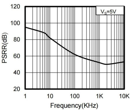
Figure 2. Power-Supply Rejection Ratio vs Frequency
