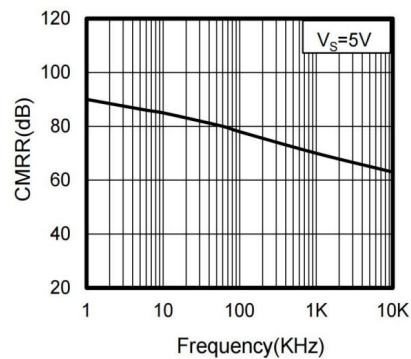
Figure 1. Common-Mode Rejection Ratio vs Frequency
