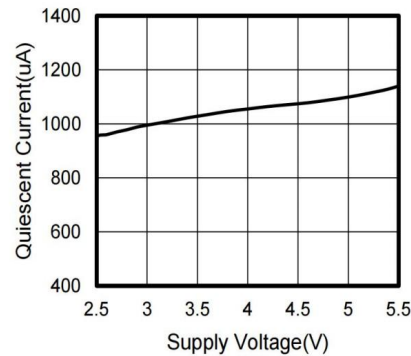
Figure 3. Quiescent Current vs Supply Voltage
