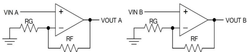
Figure 7. Schematic Representation
