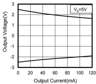
Figure 4. Output Voltage vs Output Current
