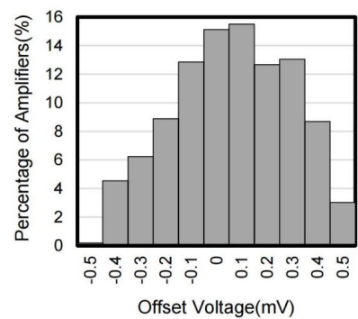
Figure 6. Offset Voltage Production Distribution
