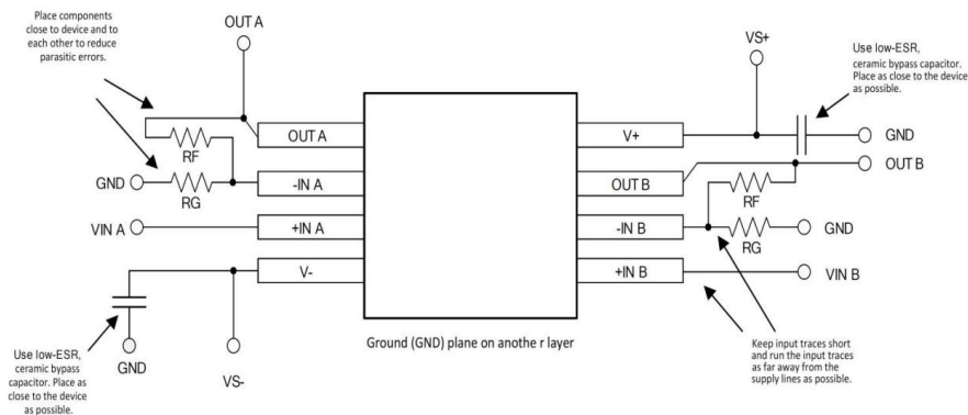
Figure 8. Layout Example
