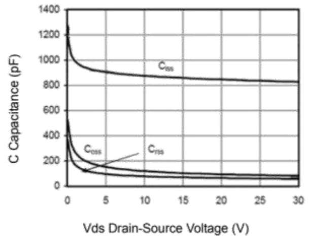
Capacitance vs.Vds
