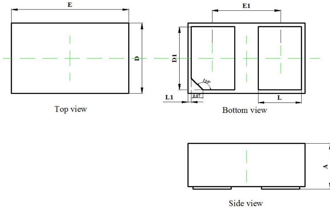
DFN1006Package Outline
