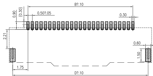
RECOMMENDED PCB PATTERN DIM.
