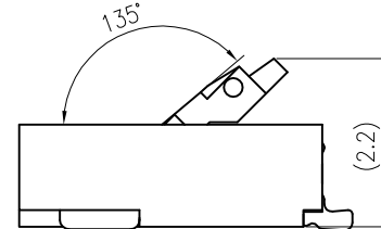
COVER OPEN STATE
