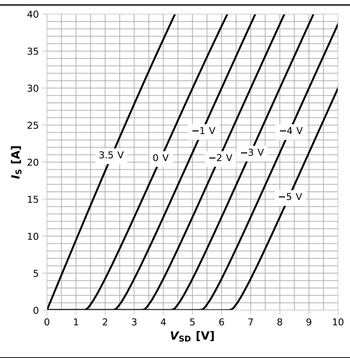
Diagram 16: Typ. channel reverse characteristics
