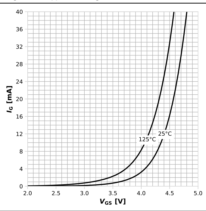
Diagram 14: Typ. transfer gate current characteristic
