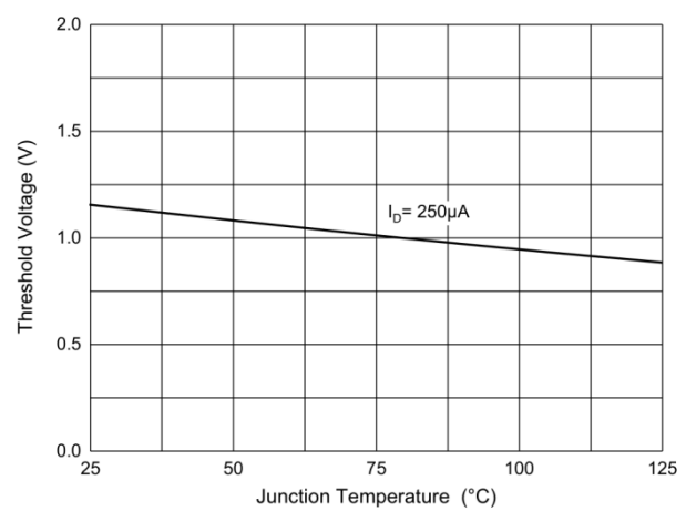
Threshold Voltage
