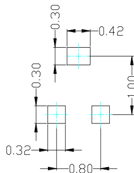
Soldering Pattern
