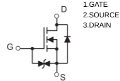
Equivalent Circuit
