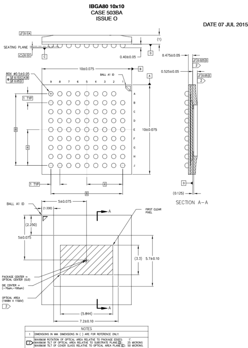
Figure 18: 80iBGA 10x10 Package Diagram (Case 503BA)
