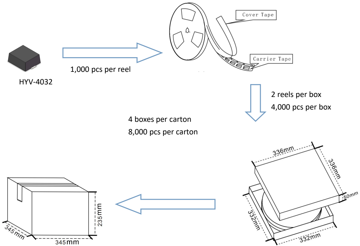
Tape and reel data(Units:mm)
