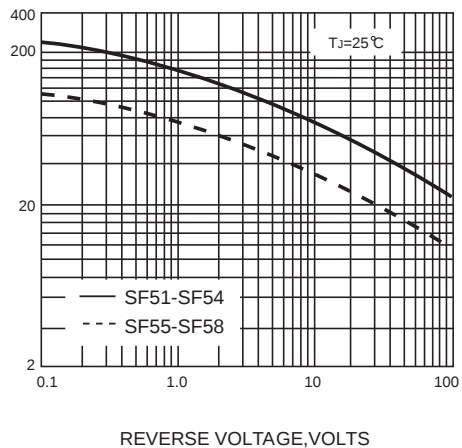
FIG. 5-TYPICAL JUNCTION CAPACITANCE
