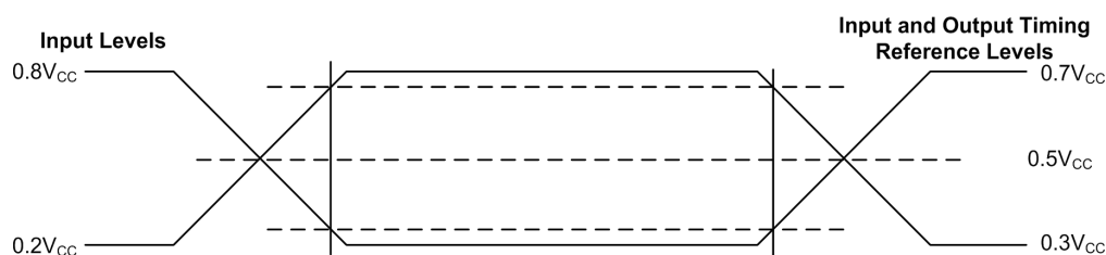
Figure 10.3 AC Measurement I/O Waveform
