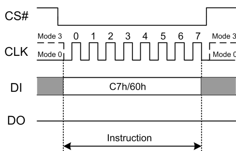
Figure 9.8 Chip Erase Instruction
