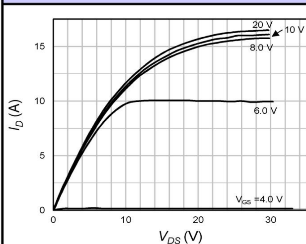
Fig.1 On-Region Characteristics.
