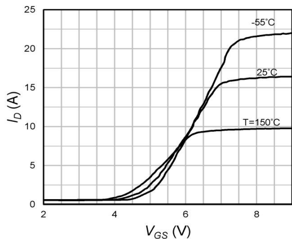
Fig.5 Transfer Characteristics
