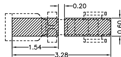
RECOMMENDED METAL MASK TOLERANCE: ±0.05
