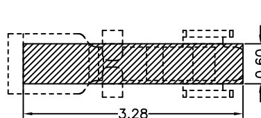
RECOMMENDED PCB LAYOUT TOLERANCE: ±0.05
