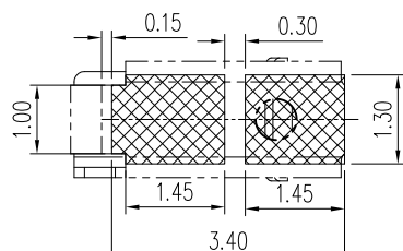
RECOMMENDED PCB LAYOUT TOLERANCE: ±0.05MM (FOR REFERENCE ONLY)
