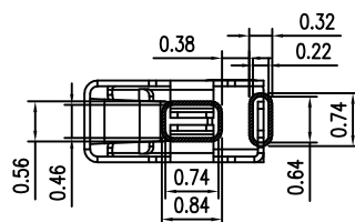
RECOMMENDED PCB LAYOUT TOLERANCE ±0.05 (焊盘推荐图)
