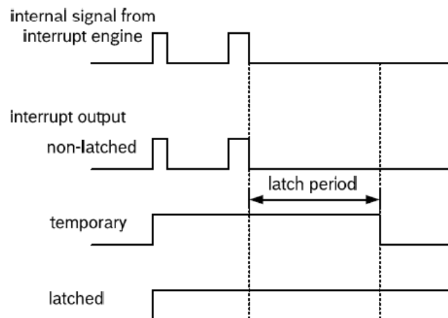
Figure 3: Interrupt mode
