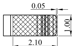
RECOMMENDED PCB LAYOUT TOLERANCE:±0.05MM (FOR REFERENCE ONLY)
