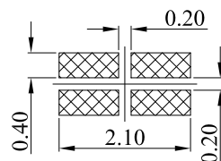
METAL MASK T=0.08 TOLERANCE:±0.05MM (FOR REFERENCE ONLY)
