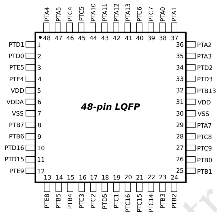
Figure 19: 48-pin LQFP Package
