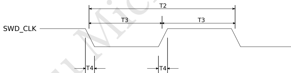
Figure 16: SWD Clock Timing
