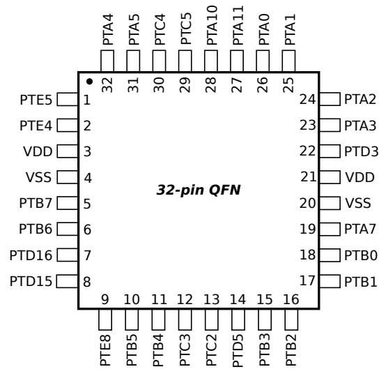
Figure 21: 32-pin QFN Package
