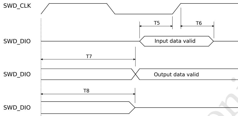
Figure 17: SWD Data Timing
