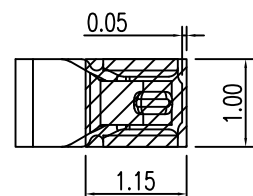
RECOMMENDED PCB LAYOUT TOLERANCE±0.05(焊盘推荐图)
