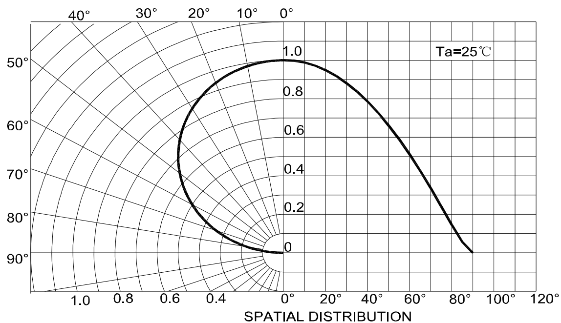
Radiation diagram
