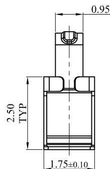
METAL MASK T=0.08 TOLERANCE:±0.05MM (FOR REFERENCE ONLY)
