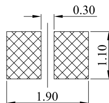
METAL MASK T=0.08
