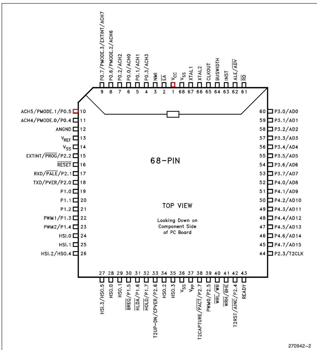
Figure 4. 68-Lead QFN Package
