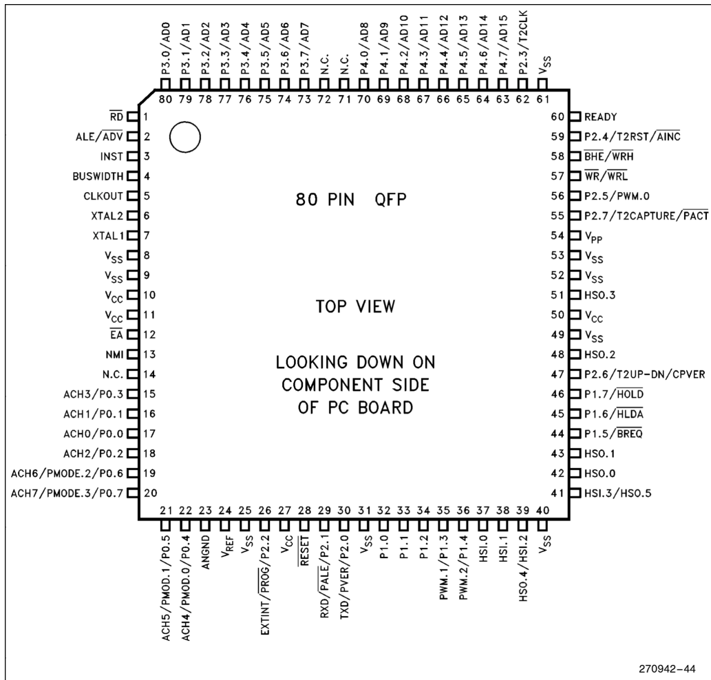
Figure 6. 80-Pin QFP Package
