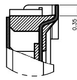
Detail B Scale 4 : 1
