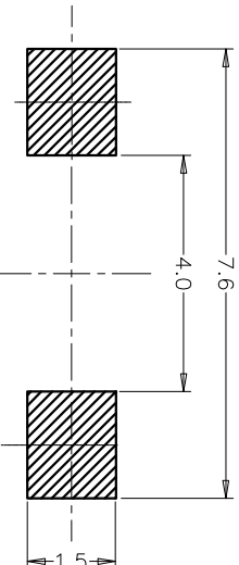
RECOMMENDED P.C.B. LAYOUT
