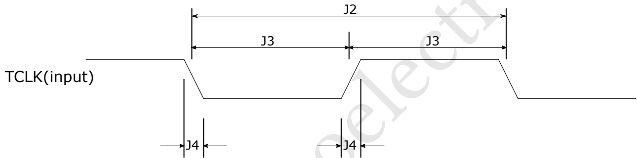
Figure 16: JTAG Clock Timing
