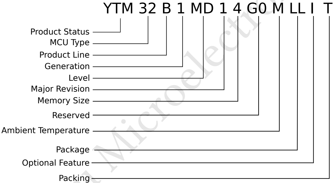
Figure 2: Part Numbers Field
