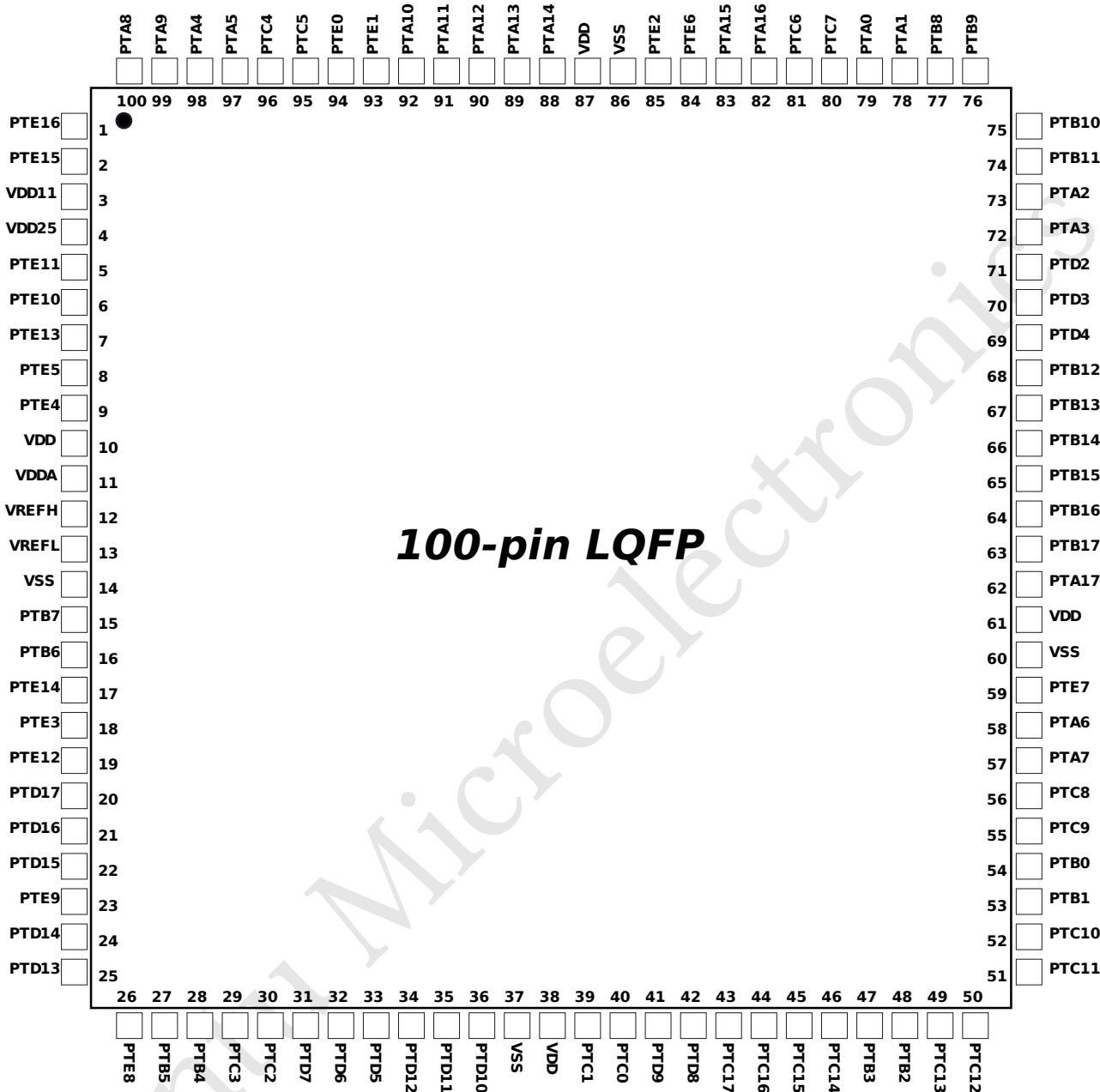
Figure 18: 100-pin LQFP Package
