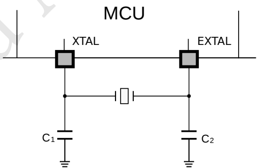
Figure 7: FXOSC Diagram
