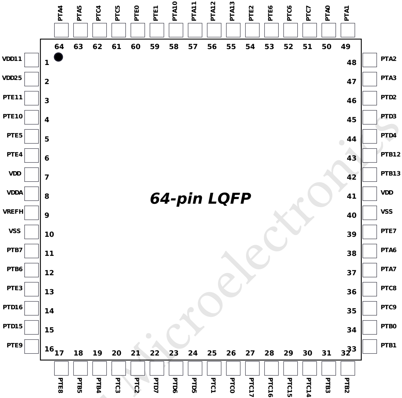
Figure 19: 64-pin LQFP Package
