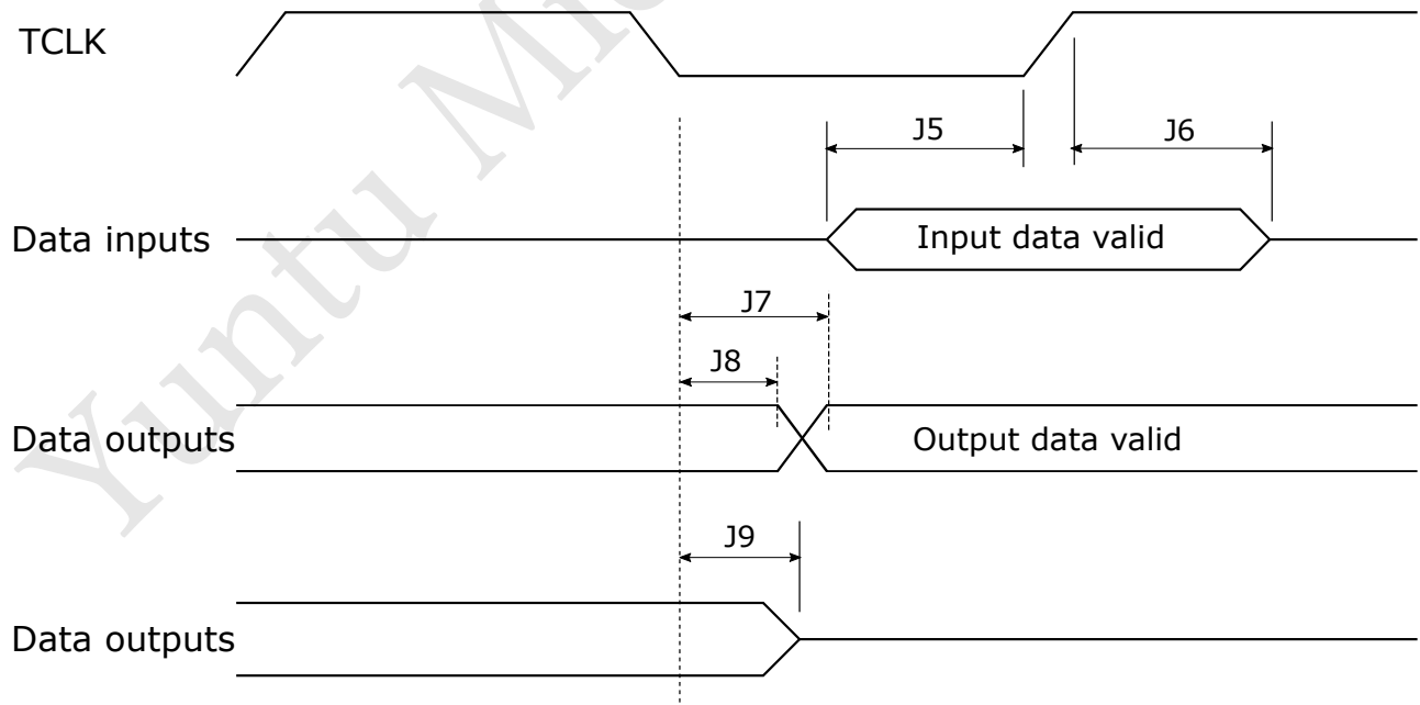
Figure 17: JTAG Data Timing
