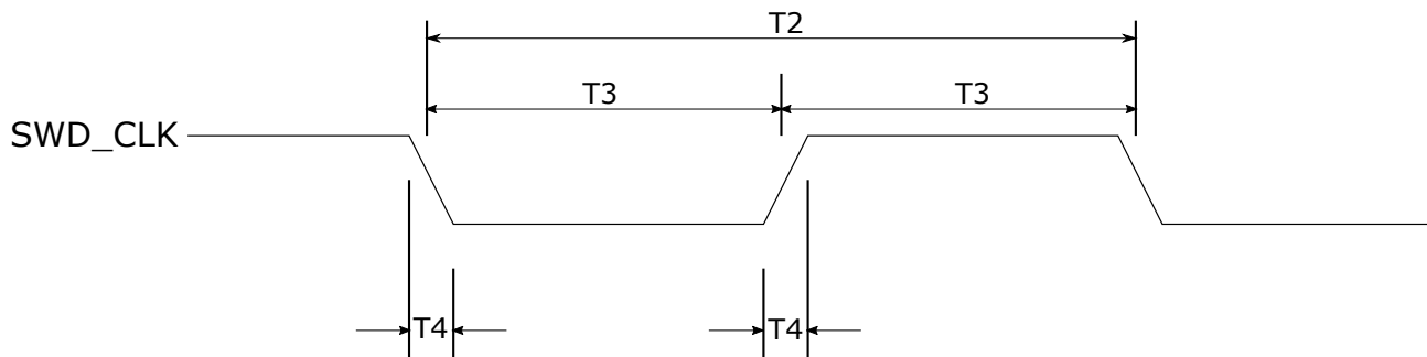
Figure 14: SWD Clock Timing
