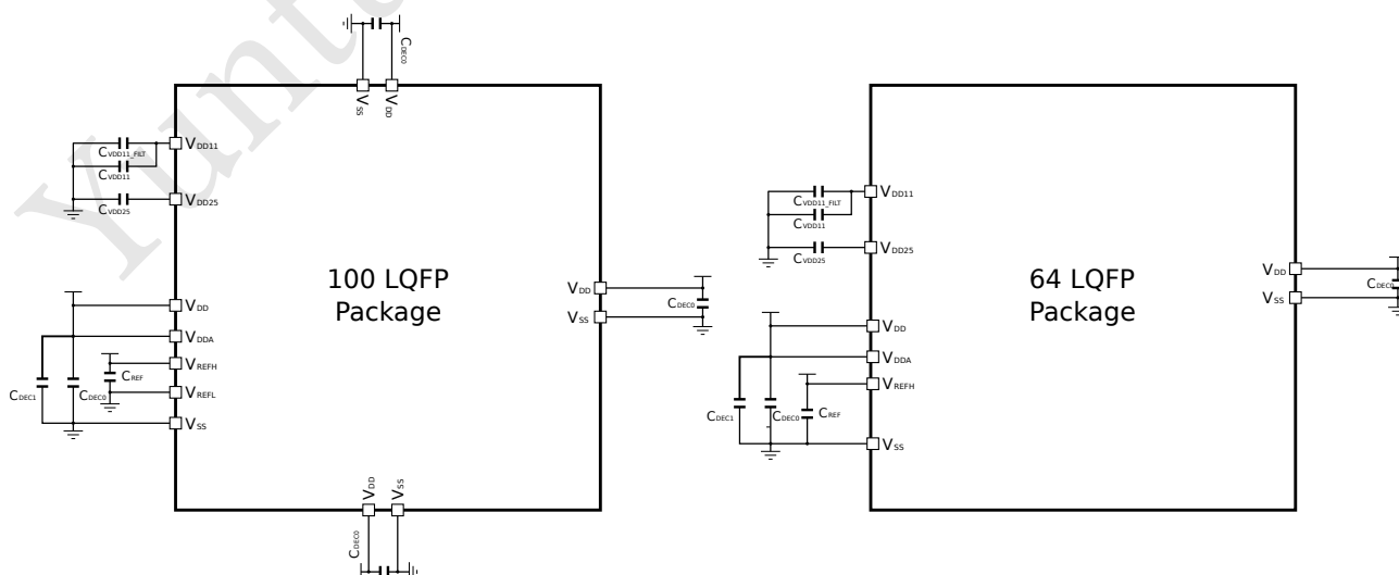
Figure 3: Pinout Decoupling
