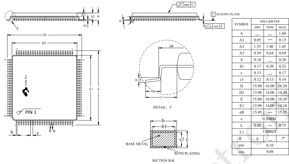
Figure 20: 100-pin LQFP
