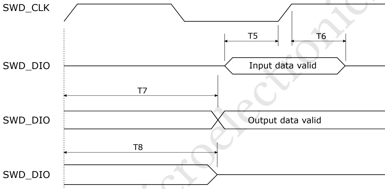
Figure 15: SWD Data Timing
