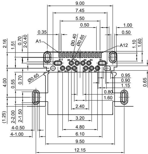
RECOMMENDED P.C.B. LAYOUT TOLERANCE UNSPECIFIED ±0.05mm (TOP VIEW)
