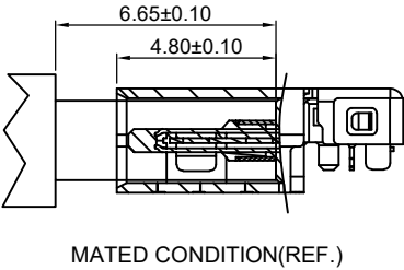
MATED CONDITION(REF.)
