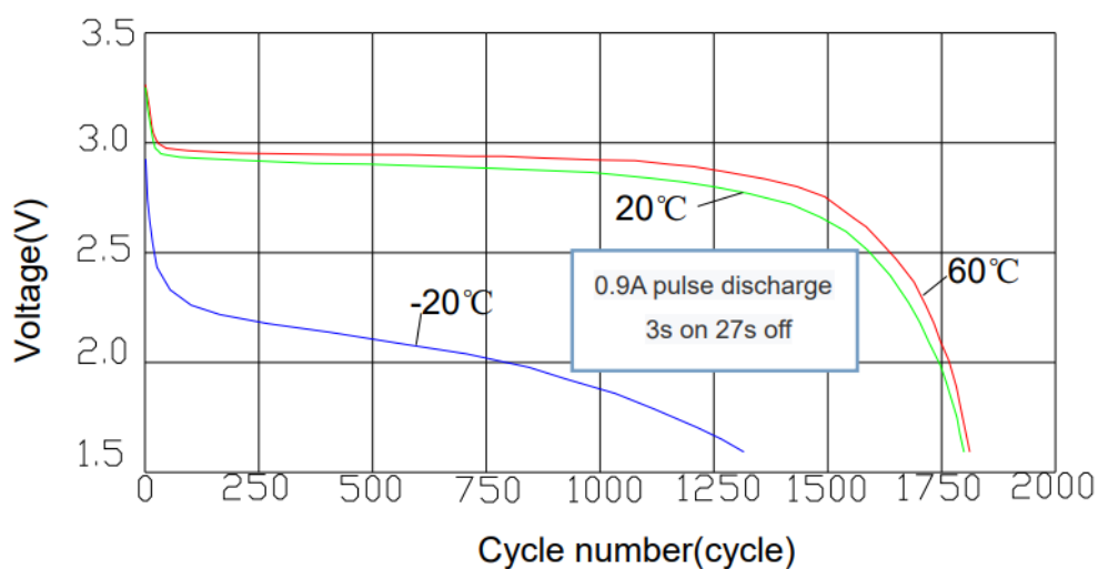
Pulse discharge characteristics
