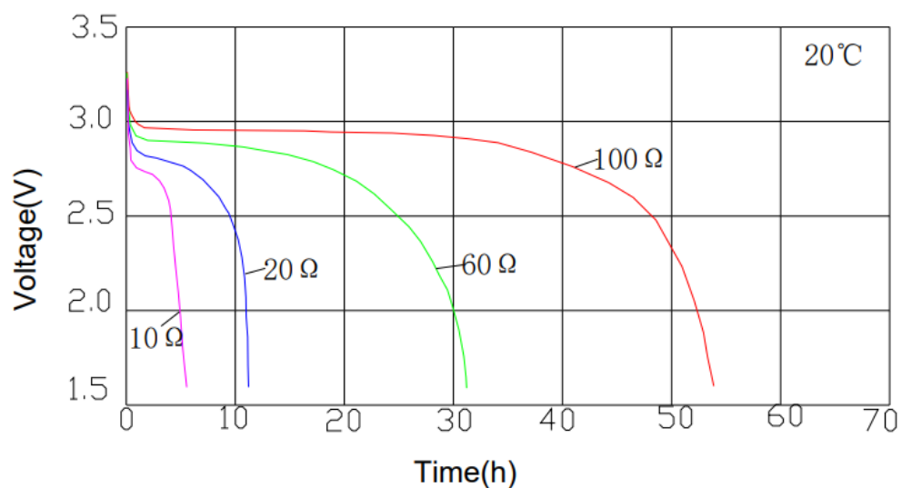
Typical discharge characteristics
