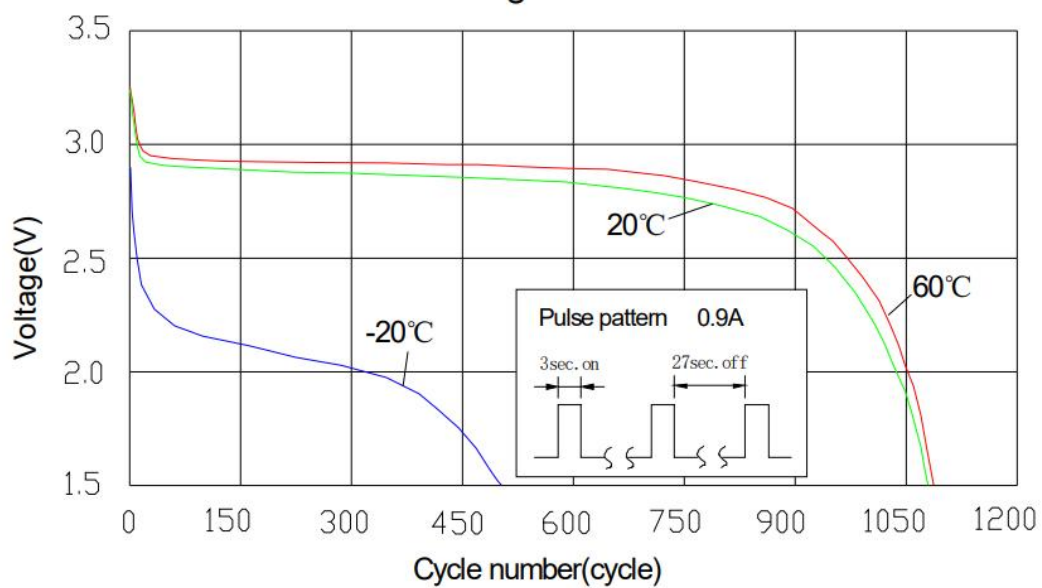
Pulse discharge characteristics
