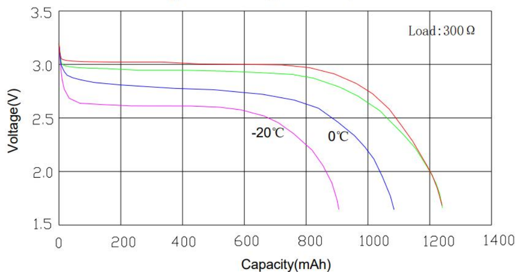
Typical Discharge vs. Temperature
