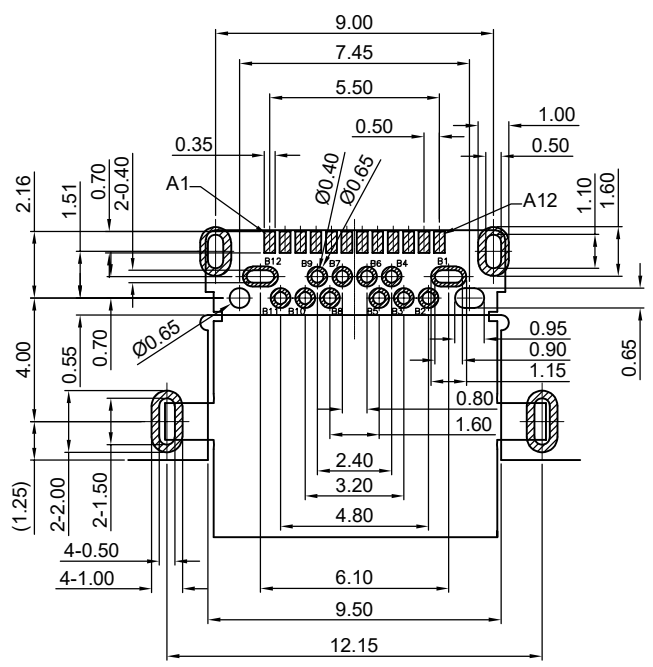
RECOMMENDED P.C.B. LAYOUT TOLERANCE UNSPECIFIED ±0.05mm
