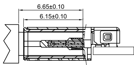
Mated Condition(REF.)
