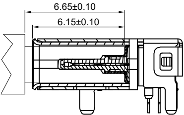
MATED CONDITION(REF.)
