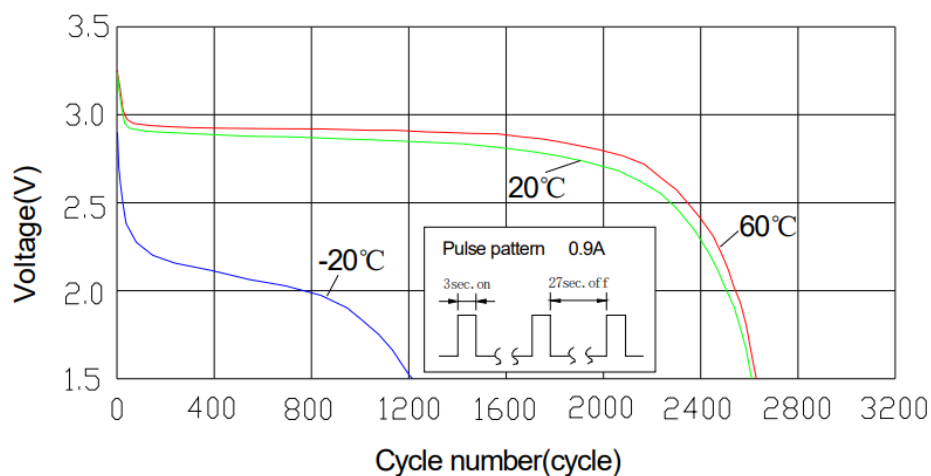
Pulse discharge characteristics
