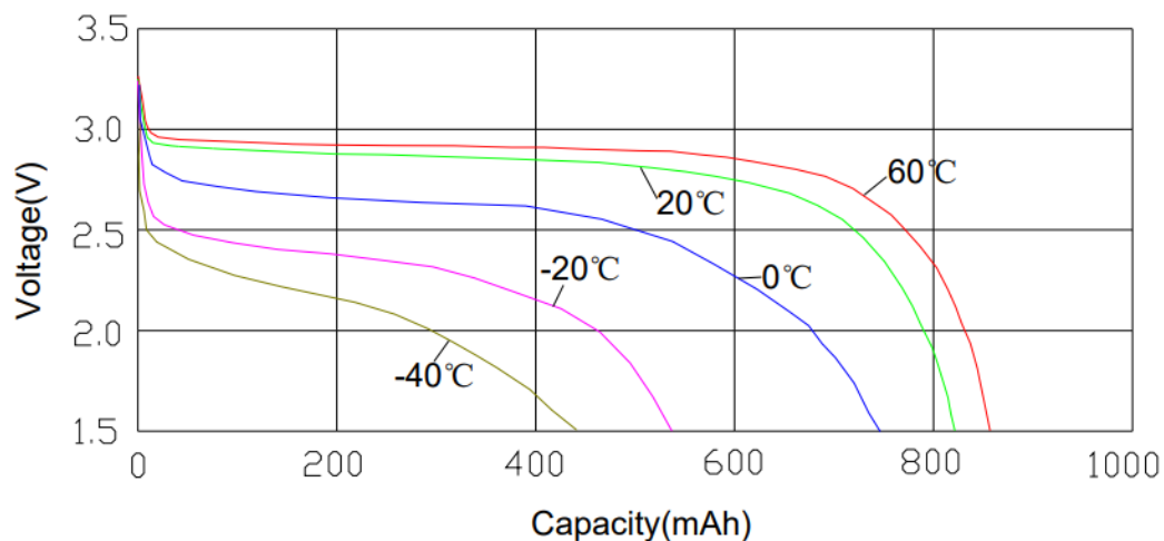
Temperature characteristics(10mA)
