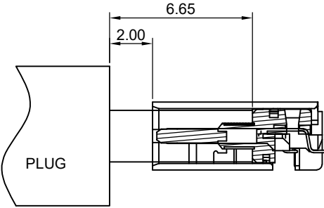
AFTER MATING
