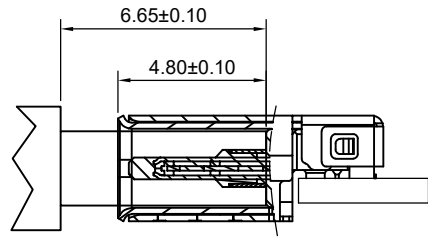
Mated Condition(REF.)
