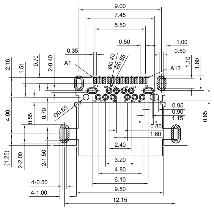
RECOMMENDED P.C.B. LAYOUT TOLERANCE UNSPECIFIED ±0.05mm
