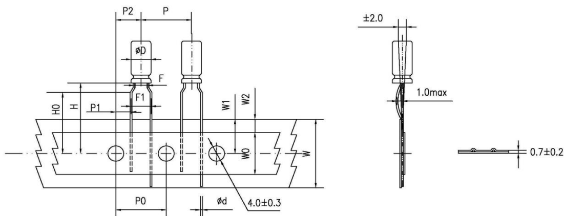
DIMENSIONS(mm)
