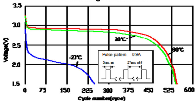
Pulse discharge characteristics
