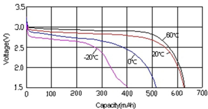
Temperature characteristics(10mA)
