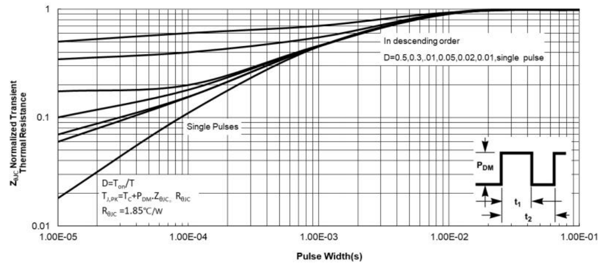
Figure 13. Maximum Effective Transient Thermal Impedance, Junction-to-Case
