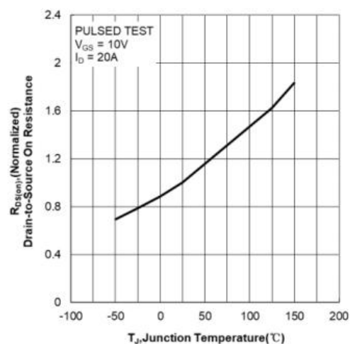
Figure 8. Normalized On Resistance vs Junction Temperature
