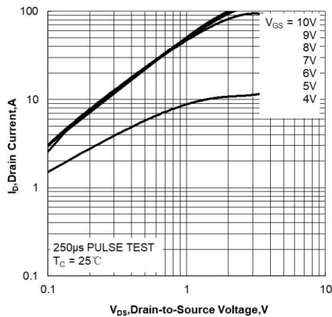
Figure 1. Output Characteristics
