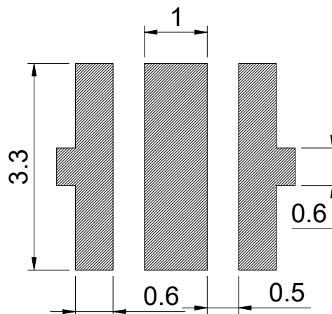
Recommend Pad Layout
