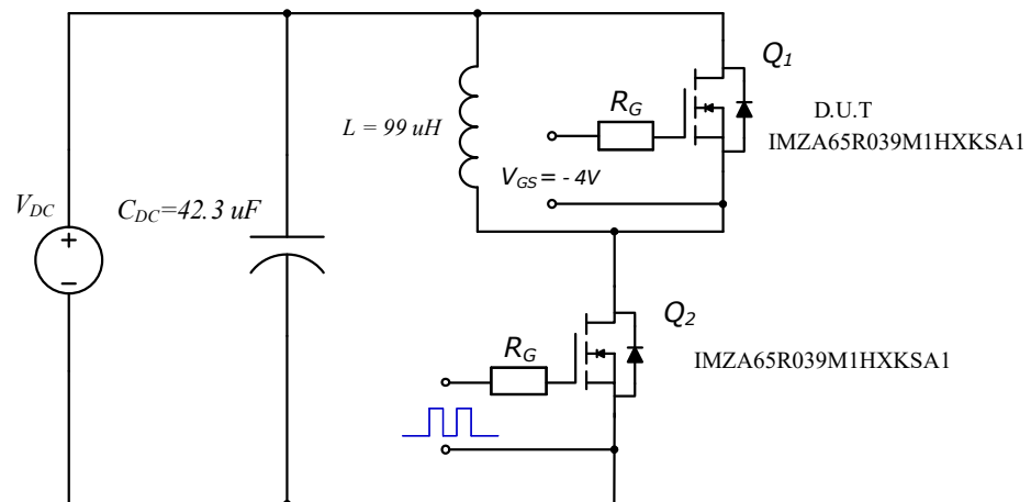
Figure 27. Body Diode Recovery Test Circuit
