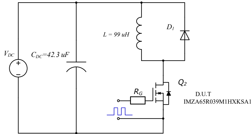
Figure 26. Clamped Inductive Switching Waveform Test Circuit
