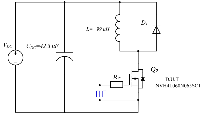
Figure 26. Clamped Inductive Switching Waveform Test Circuit
