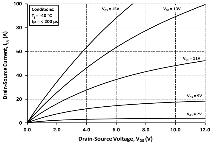
Figure 1. Output Characteristics T_j = -40^\circ\text{C}
