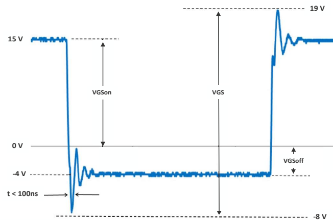
Figure 28. V_{GS} Waveform Example
