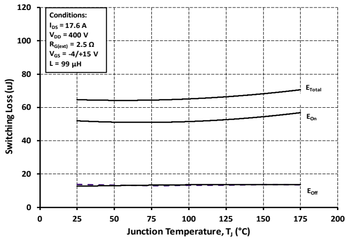
Figure 24. Clamped Inductive Switching Energy vs. Temperature
