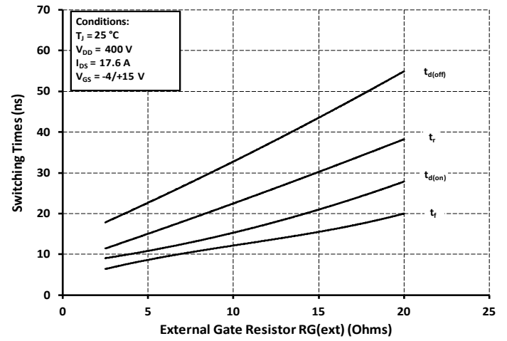
Figure 25. Switching Times vs. R_{G(ext)}
