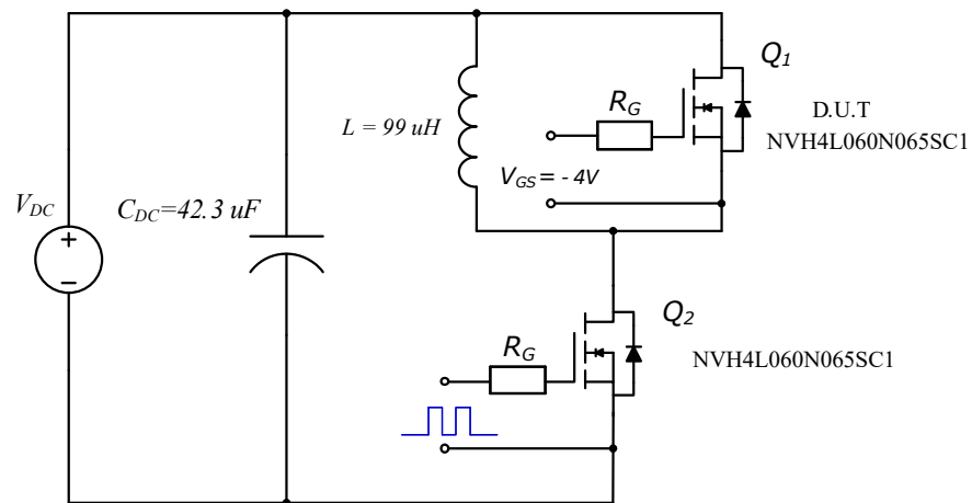
Figure 27. Body Diode Recovery Test Circuit
