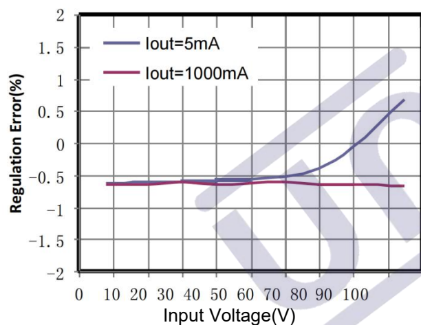
Line Regulation
