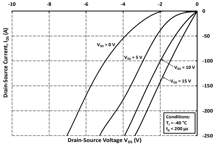
Figure 13. 3rd Quadrant Characteristic at -40\text{ }^{\circ}\text{C}
