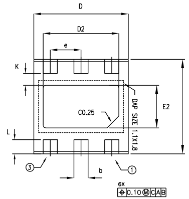
Figure 26. DFN6 (2 x 2) wettable flanks package outline
