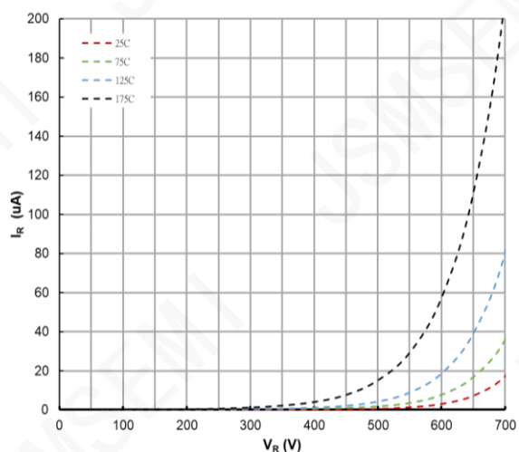
Figure 3. Reverse Characteristics
