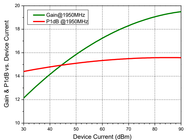
Gain & P1dB vs. Current
