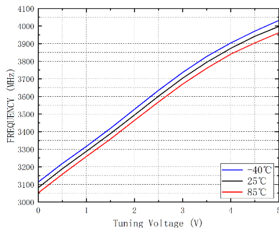
Frequency vs. Tuning Voltage vs. Temperature
