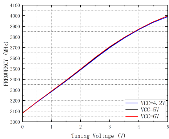
Frequency vs. Tuning Voltage vs. Operating Voltage
